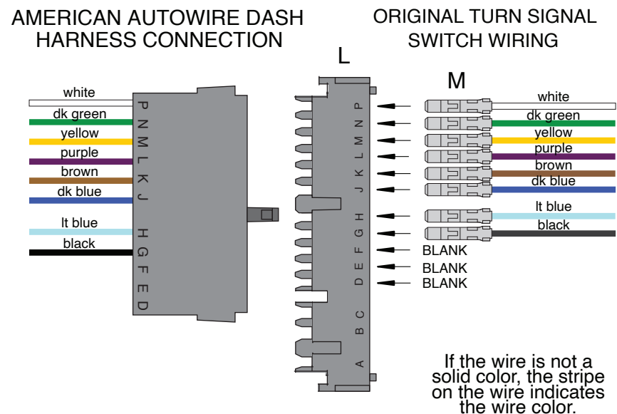
AAW Turn Signal Switch Wires to Stock Steering Columns.
